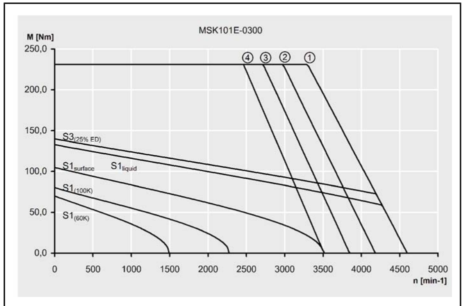
Fig.4-113: Speed-torque characteristic of MSK101E-0200
